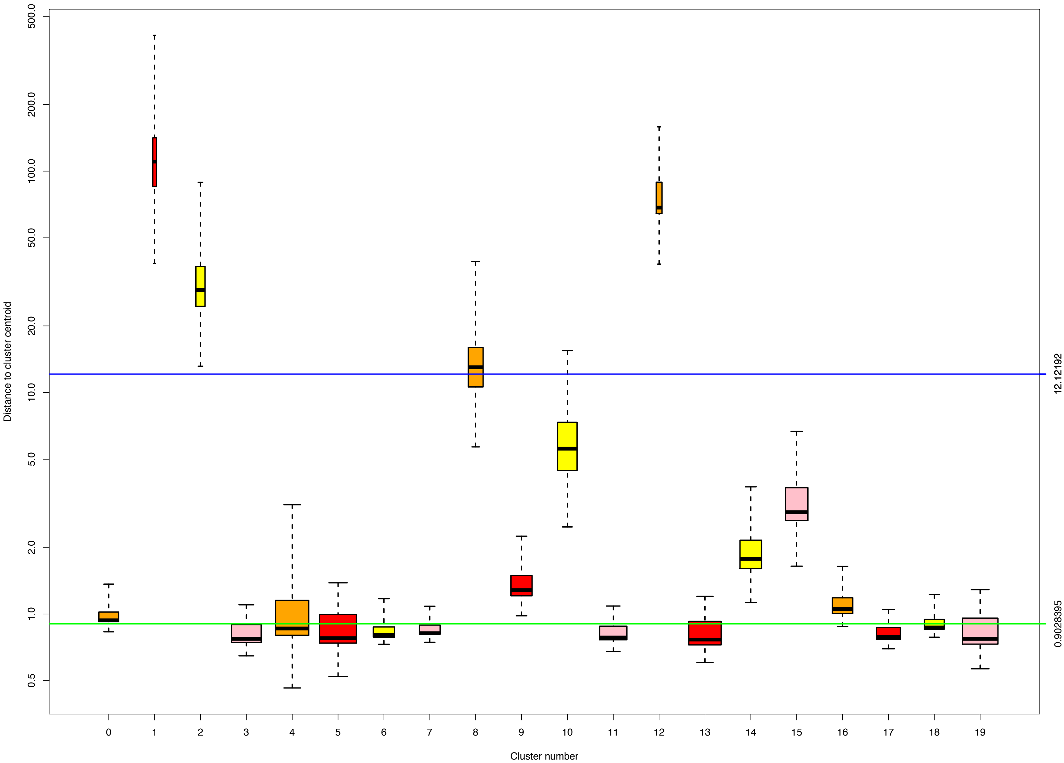
Mahout KMeans: Run 1
